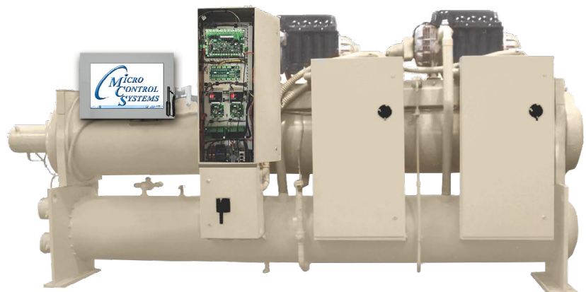
New Controls installed in existing cabinet. New Touchscreen
